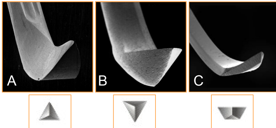
Figure 42. Cutting needles
