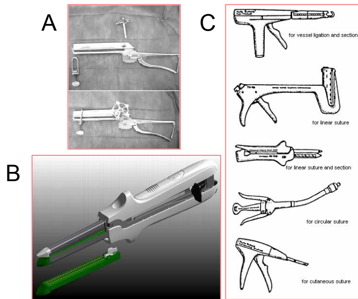
Figure 33. Staplers
